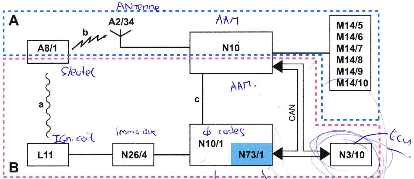
Illustration of the principle (gasoline engine)
